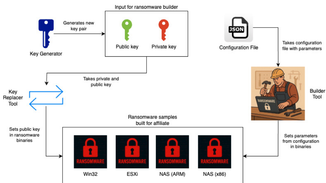
Figure 2: The software components in the Playboy toolchain and how they are related.
