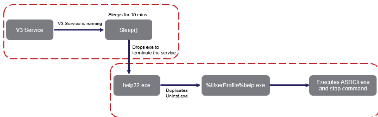
Figure 11: Process to disable V3 service.
