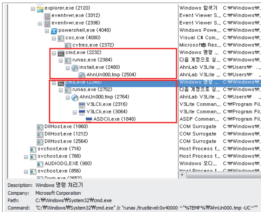
Figure 10: Process structure of uninstalling.
