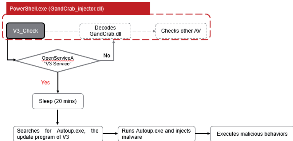
Figure 13: Evasive process used by GandCrab to bypass V3 Lite .
